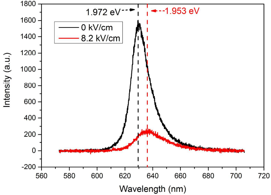
Figure S3. Highest quenching achieved by applying high electric field.
