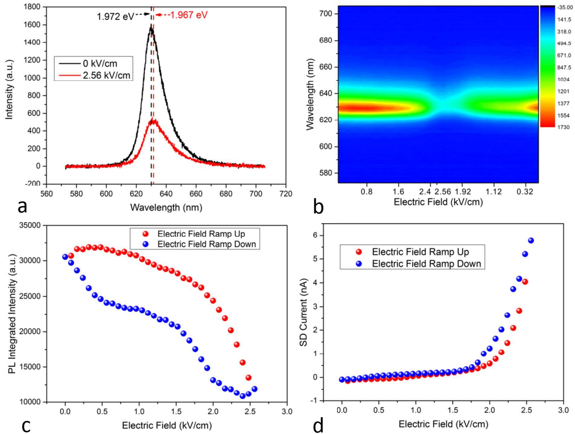
Figure S1. Another example of PL quenching from monolayer WS 2 . a) Typical PL spectra under two different electric fields, 0 kV/cm and 2.56 kV/cm. b) Colour contour map of PL spectra under lateral electric field. c) PL integrated intensity versus electric field. d) I-V trace during laser illumination and PL measurement. Red dots: electric field ramps up. Blue dots: electric field ramps down.
