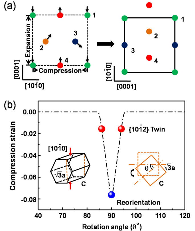
FIG. 2. (Color online) Lattice reorientation from [10\bar{1}0] -oriented hcp to [0001] -oriented hcp in terms of a displacive transformation mechanism. (a) The lattice reorientation can be described in terms of a shuffle (displacement) and a global shape change. The arrows show the shuffle directions for the four atoms. (b) Comparison of the compressional strain versus reorientation angles for the 90^\circ reorientation and \{10\bar{1}2\} twins. The left schematic shows compression direction on the hcp unit cell. The (\bar{1}210) plane shown as a dotted line rotates by angle \theta (right schematic). A rotation of 84.6^\circ gives rise to \{10\bar{1}2\} twins and 90^\circ leads to the reoriented domains discussed in this work.
