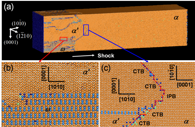
FIG. 1. (Color online) Microstructure from NEMD shock simulations of shocked Ti single crystal samples. (a) Shocked samples with particle velocity, u_p = 7.5 m/s along [10\bar{1}0] direction containing approximately 3.0 million atoms in volume 24 \text{ nm} \times 24 \text{ nm} \times 200 \text{ nm} after 18.0 ps. The initial hcp \alpha phase, reoriented hcp \alpha' phase, and transformed \omega phase are shown with a trapezoidal-shaped domain boundary separating \alpha and \alpha' . (b) Coexisting [0001] \alpha' and transformed \omega phases. (c) The 90^\circ domain boundary between \alpha and \alpha' from the cross section (blue rectangle) in (a) consists of an IPB, CTBs, and dislocation kinks and disconnections.
