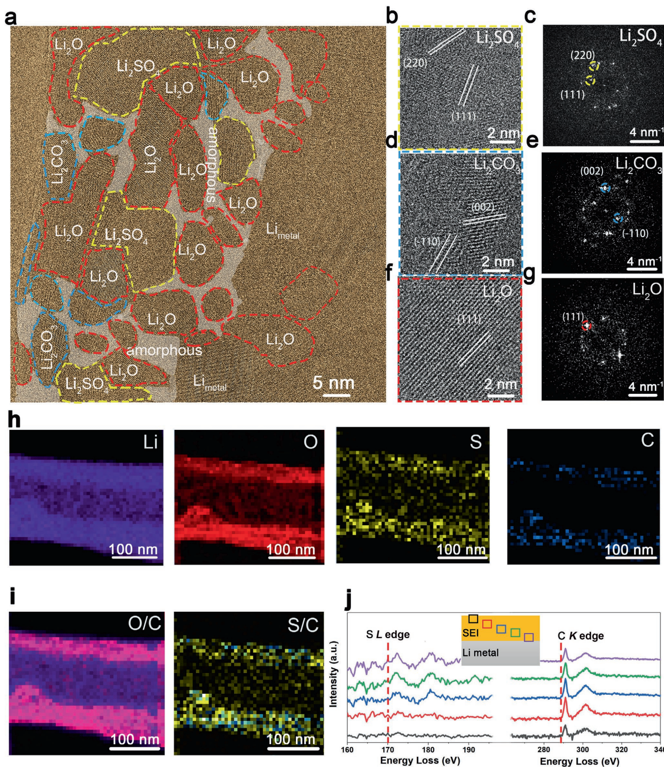
Figure 5. Cryo-HRTEM images of SEI structure in (EC/DEC+2% PS) Electrolyte. a) HRTEM image of the SEI on lithium dendrites acquired using electron dosage \approx 100 \text{ e}^- \text{ \AA}^{-2} . [2] b,c) HRTEM and FFT of \text{Li}_2\text{SO}_4 crystal. d,e) \text{Li}_2\text{CO}_3 crystal. f,g) \text{Li}_2\text{O} crystal. h) EELS elemental mapping shows the distribution of lithium (purple), oxygen (red), sulfur (yellow), and carbonate (blue) in the lithium dendrites. Due to increased thickness, the middle region of the dendrite has less EELS signal. i) The combination of carbonate, oxygen and sulfur EELS elemental mapping. j) The EELS of S and C K-edge acquired from \text{Li}_{\text{Metal}} to SEI surface.
