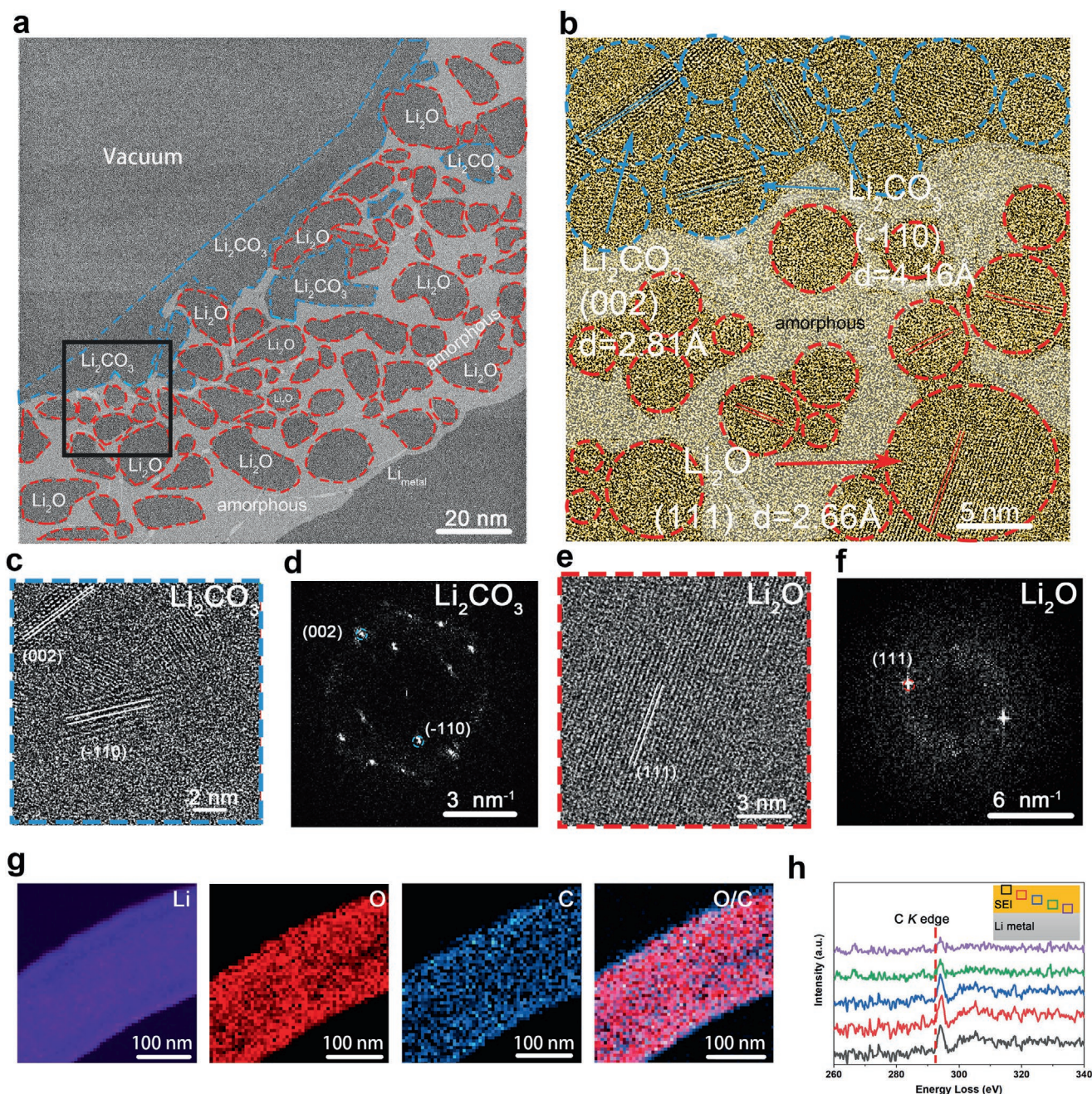
Figure 3. Cryo-TEM images and elemental compositions of SEI structure in the blank (EC/DEC) electrolyte acquired using electron dosage \approx 100 \text{ e} \text{ \AA}^{-2} . [2] a) Phase map of the SEI. b) Magnified HRTEM image of the area marked by the black square in (a). c, d) HRTEM and FFT of \text{Li}_2\text{CO}_3 crystal. e, f) HRTEM and FFT of \text{Li}_2\text{O} crystal. g) EELS elemental mapping shows the distribution of lithium (purple), oxygen (red), carbonate (blue), and composite mapping of the lithium dendrites. h) The EELS of carbon (C) K-edge acquired from \text{Li}_{\text{Metal}} to SEI surface in (EC/DEC) electrolyte, respectively.
