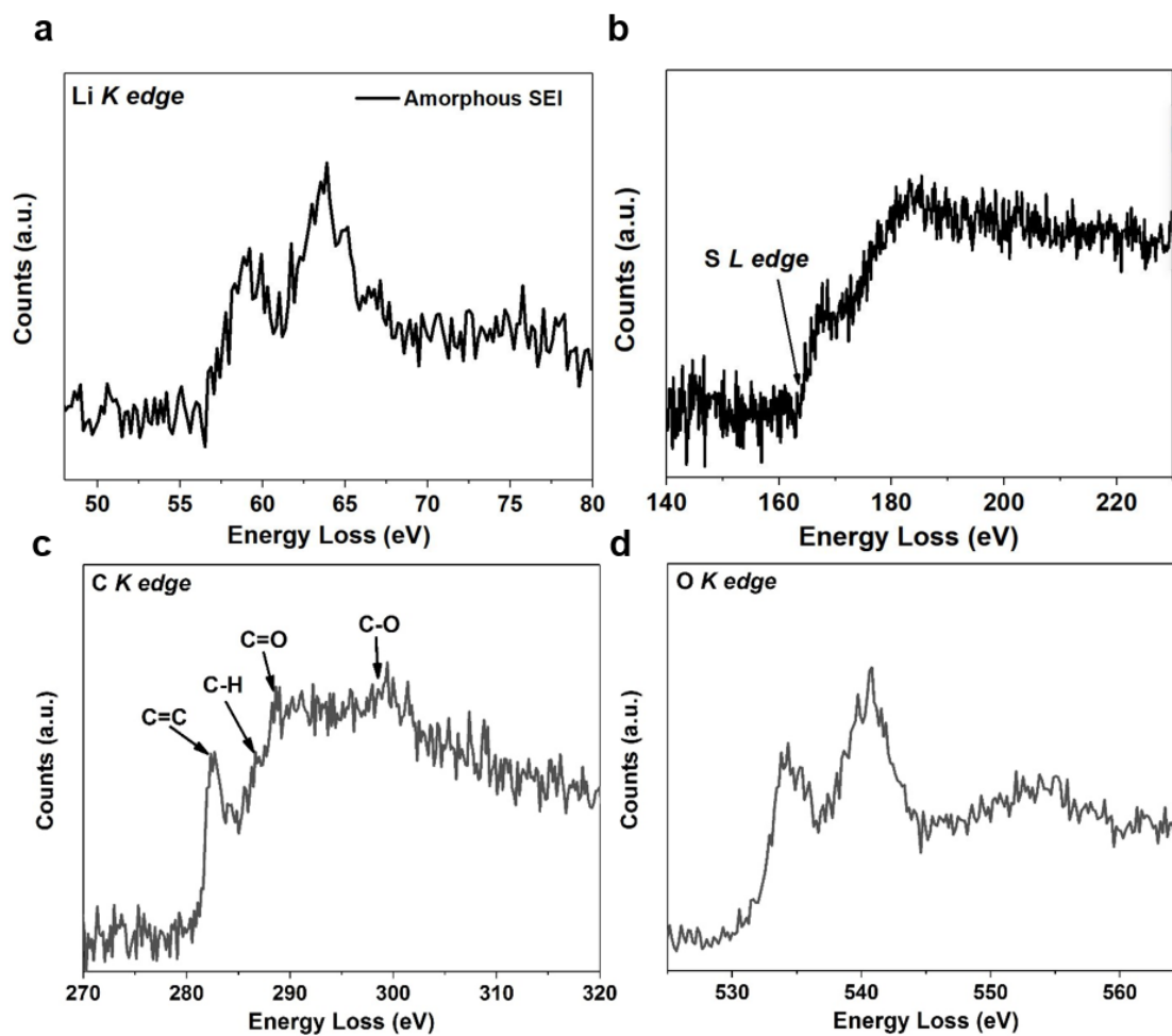
Fig.S5 EELS acquired from the amorphous phase in the SEI. a, Li K-edge. b, S L-edge. c, C K-edge. d, O K-edge. We can see clearly the EELS signature from Li, C, O, and S in the EELS. The Li K edge shows a oxidized signature and the C peaks shows the possible content of C=C, C-H, C=O, and C-O peaks.
