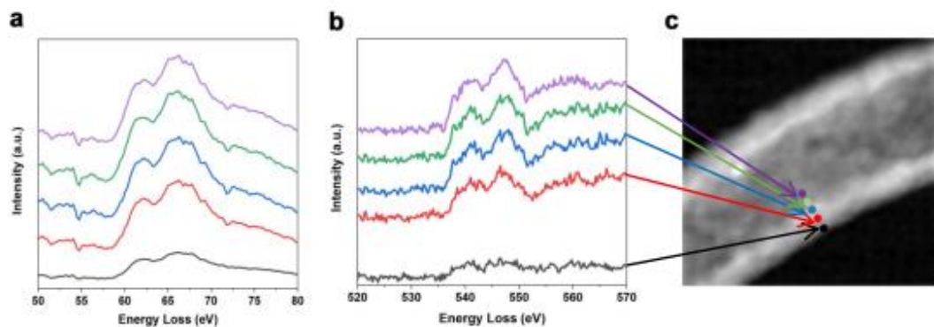
Fig.S2 The EELS of Li and O K-edge acquired from the lithium, interface, SEI and surface in (EC/DEC) electrolyte respectively, the black line represent the surface and the purple line represent the lithium. a , the Li K-edge acquired from the different place on dendrite in (EC/DEC) electrolyte. b , the O K-edge acquired from the different place on dendrite in (EC/DEC) electrolyte. c , the location corresponding to the spectrum from (a) and (b) .
