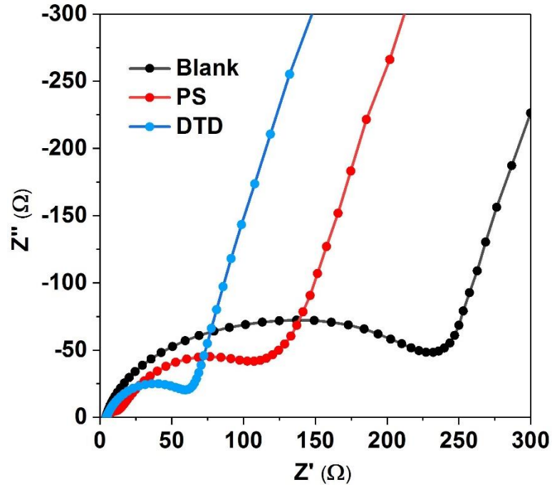
Fig. S1 The EIS plot of Li/Cu half-cells containing different electrolytes after three cycles.
