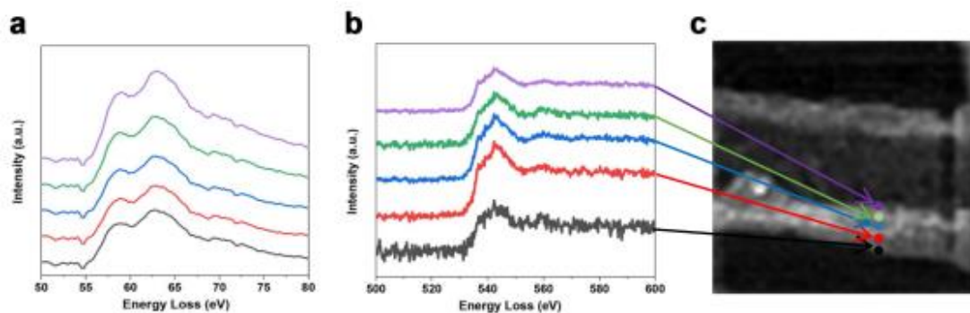
Fig.S4 The EELS of Li and O K-edge acquired from the lithium, interface, SEI and surface in (EC/DEC+ 2%PS) electrolyte respectively, the black line represent the surface and the purple line represent the lithium. a , the Li K-edge acquired from the different place on dendrite in (EC/DEC+ 2%PS) electrolyte. b , the O K-edge acquired from the different place on dendrite in (EC/DEC+ 2%PS) electrolyte. c , the location corresponding to the spectrum from (a) and (b).
