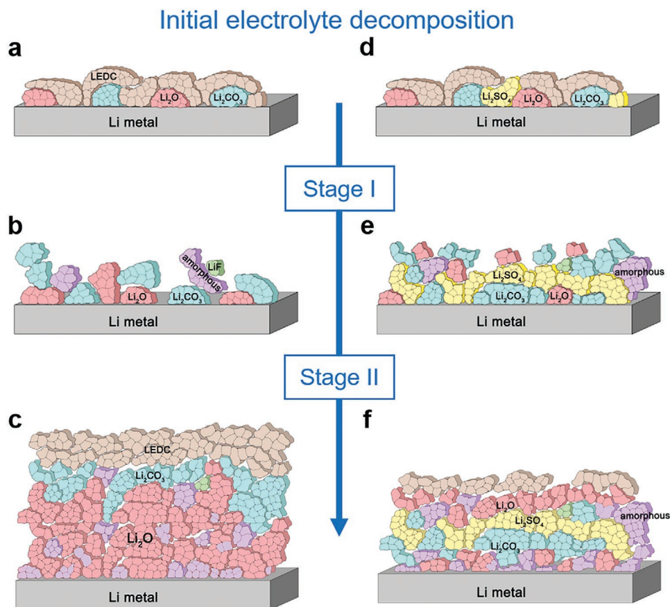
Figure 6. a–c) Schematic of SEI formation on the \text{Li}_{\text{Metal}} electrode with blank electrolyte, due to the continuous decomposition of LEDC and \text{Li}_2\text{CO}_3 , lots of lithium oxide remains on the surface of the \text{Li}_{\text{Metal}} . The \text{Li}_2\text{CO}_3 decompose once touched \text{Li}_{\text{Metal}} surface. The partial exposure of the \text{Li}_{\text{Metal}} leads to the continuous reaction. d–f) SEI formation using the DTD electrolyte additive greatly expands the stability of SEI. DTD produces \text{Li}_2\text{SO}_4 , which cover lithium carbonate and inhibit the decomposition of lithium carbonate and electrolyte.
