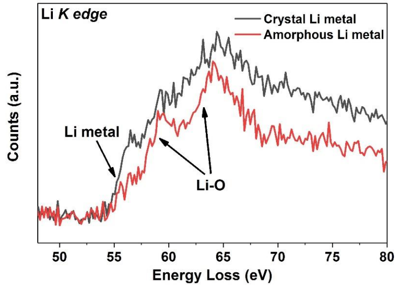
Fig.S6 The EELS fine structures of Li K edge in the amorphous region and crystal region. The amorphous Li regions shows a more significant signature of oxidized Li peak, which is due to the higher content of oxygen or sulfur inside the amorphous Li metal. The two separate peaks in the red curve are related to the bonding between Li and O atoms.
