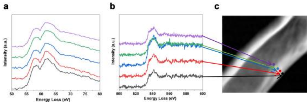
Fig.S3 The EELS of Li and O K-edge acquired from the lithium, interface, SEI and surface in (EC/DEC+ 2%DTD) electrolyte respectively, the black line represent the surface and the purple line represent the lithium. a , the Li K-edge acquired from the different place on dendrite in (EC/DEC+ 2%DTD) electrolyte. b , the O K-edge acquired from the different place on dendrite in (EC/DEC+ 2%DTD) electrolyte. c , the location corresponding to the spectrum from (a) and (b).
