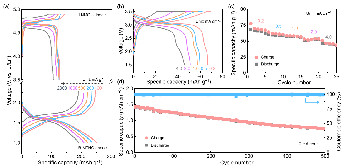
Fig. 4. (a) Galvanostatic discharge/charge profiles for \text{LiNi}_{0.5}\text{Mn}_{1.5}\text{O}_4 cathode and R-MTNO anode. (b) Galvanostatic discharge/charge profiles, (c) rate performance and (d) cycling performance of \text{LiNi}_{0.5}\text{Mn}_{1.5}\text{O}_4 \parallel R-MTNO full cells.
